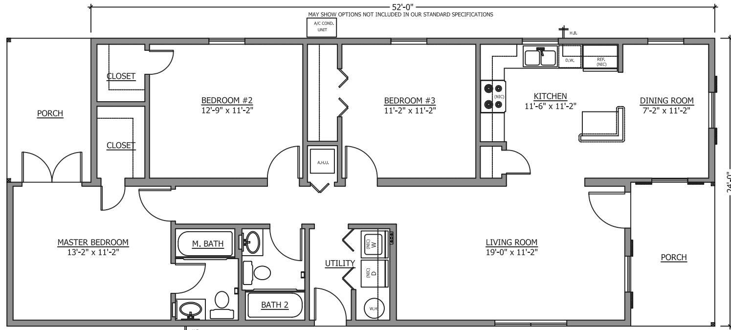
FLOOR PLAN
