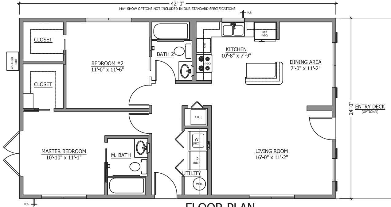
FLOOR PLAN
