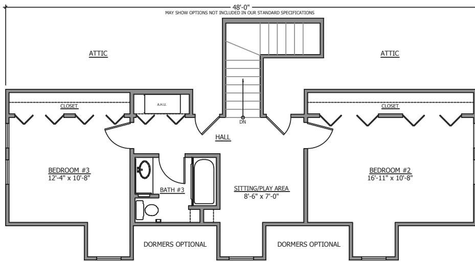
SECOND FLOOR
